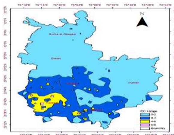
Fig. 1.12 Spatial variability of EC of groundwater used for irrigation in Kaithal district
