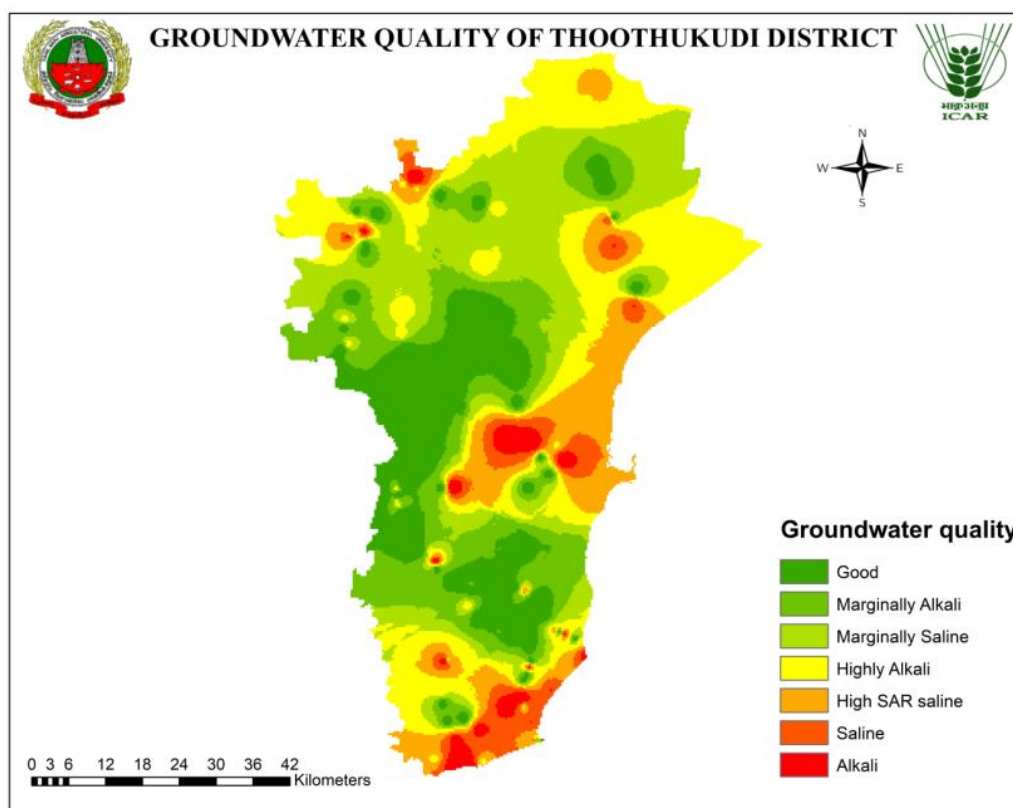
Fig. 1.20 Spatial distribution of groundwater quality categories for Thoothukudi district
