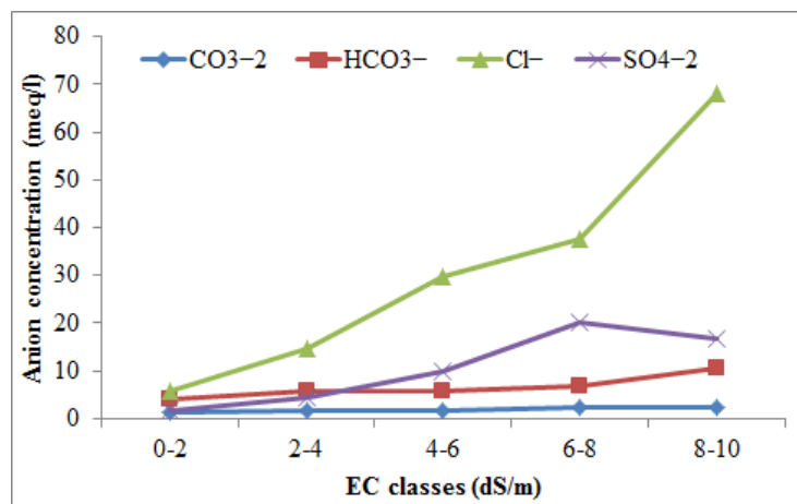
Fig. 1.10 Anions (CO 3 , HCO 3 , Cl, SO 4 ) concentration (me/l) in different EC classes of Faridabad district
