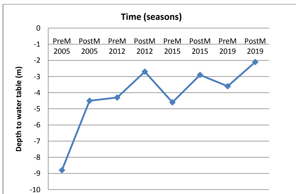
Fig. 2.3 Depth to water table with time in canal command
